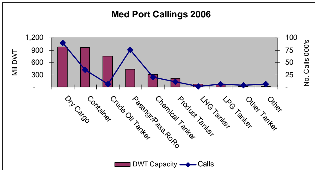
Figure 2.3 Mediterranean Calls vs Deployed Capacity
